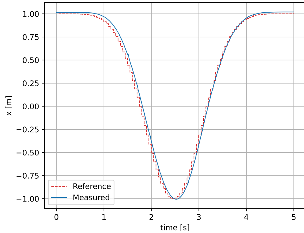
x State
