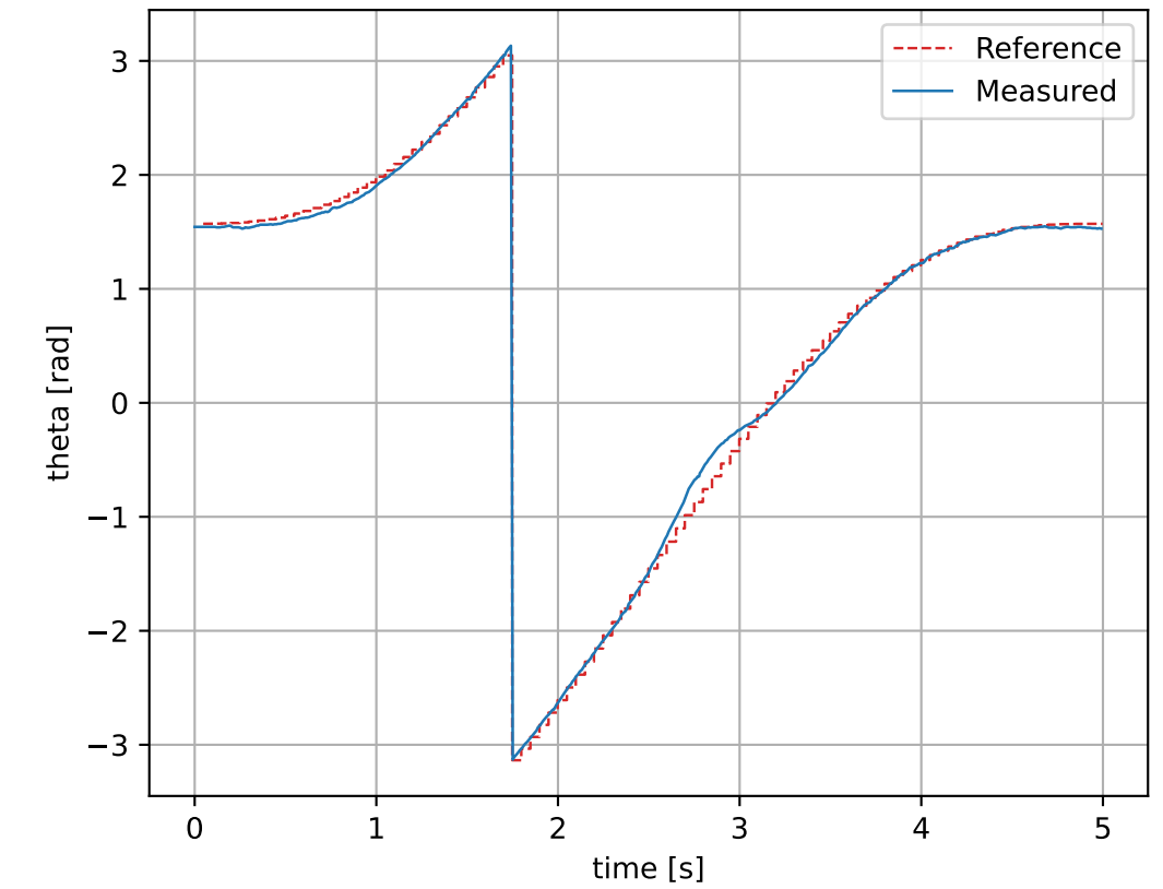
theta State
